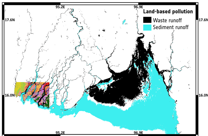
Example of land-based runoff for the Ayeyarwady Delta in Myanmar based on data from Sentinel-3 and Sentinel-2 (lower left coloured area), acquired on 22-11-2018. The Sentinel-2 data provide land use classification that may contribute to identifying potential causes of the pollution.
